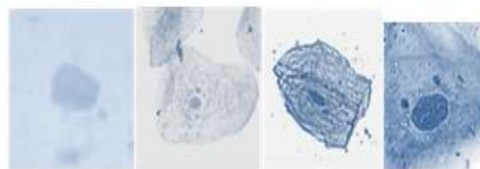
Fig. 1: Micronucleus
